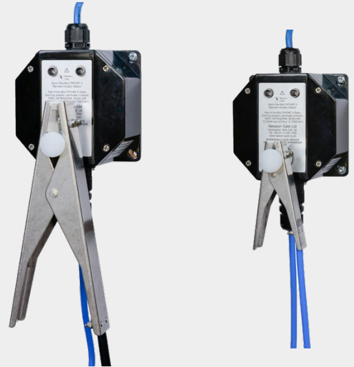
The Earth-Rite MULTIPOINT II's energy efficient remote indicator stations provide ground status indication for each individual channel. The attention grabbing high intensity GREEN LED pulses continuously when a positive ground connection is made.
